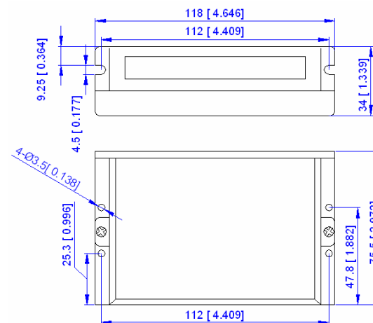
Figure 1: Mechanical specifications
