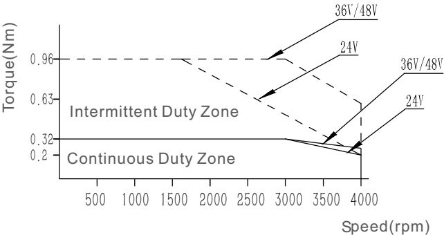
The curve of torque -speed
